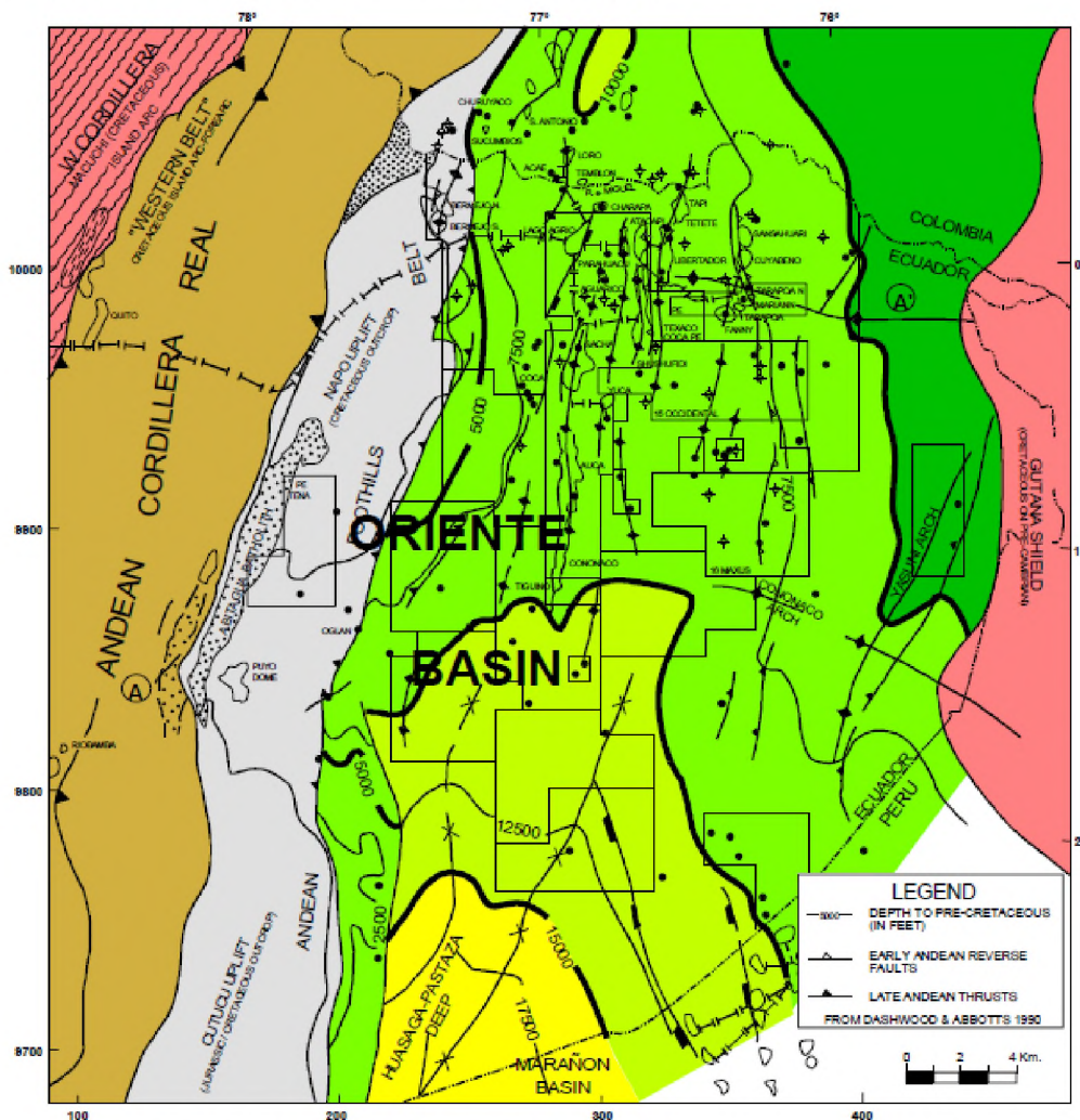
Figure: 2. Tectonic structure and location of oil wells [1,2]
